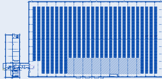
NARROW RACKING PLAN
